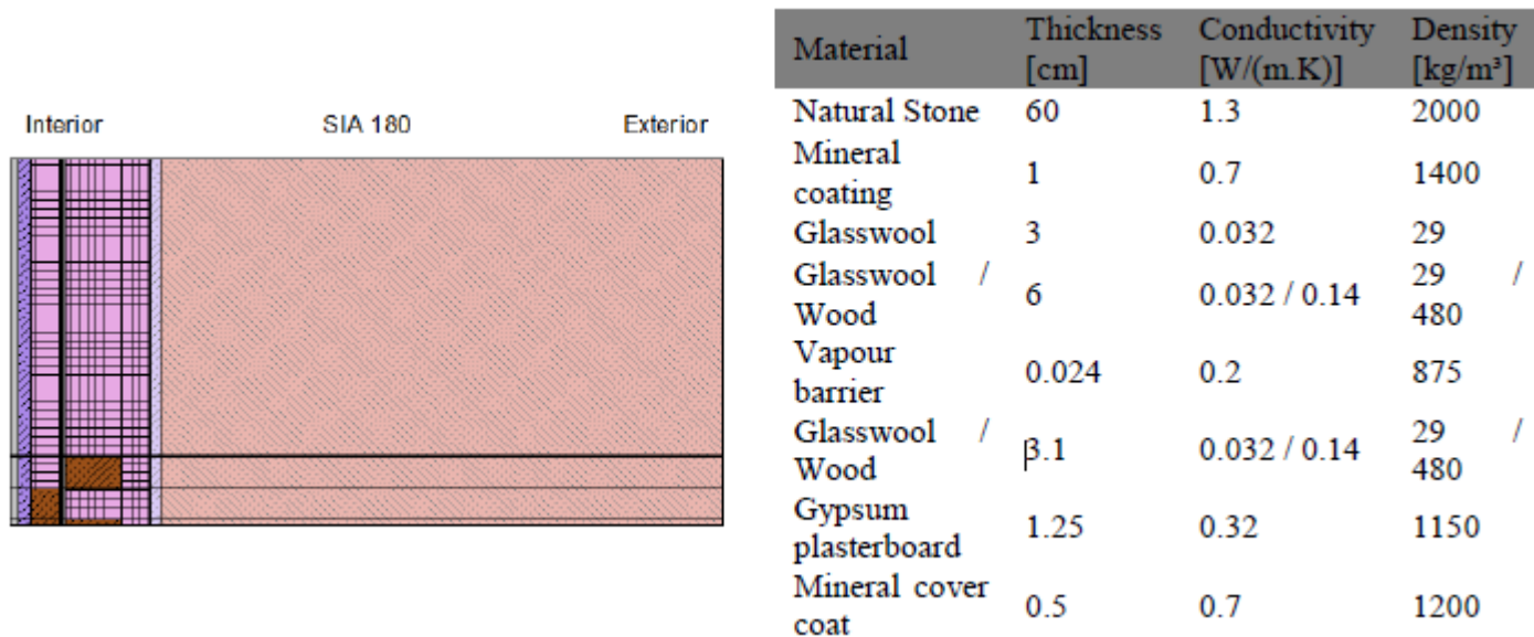
Figure 19. Stratigraphy of insulation systems n.8 (Glass Wool). From RibuildD5.1.
